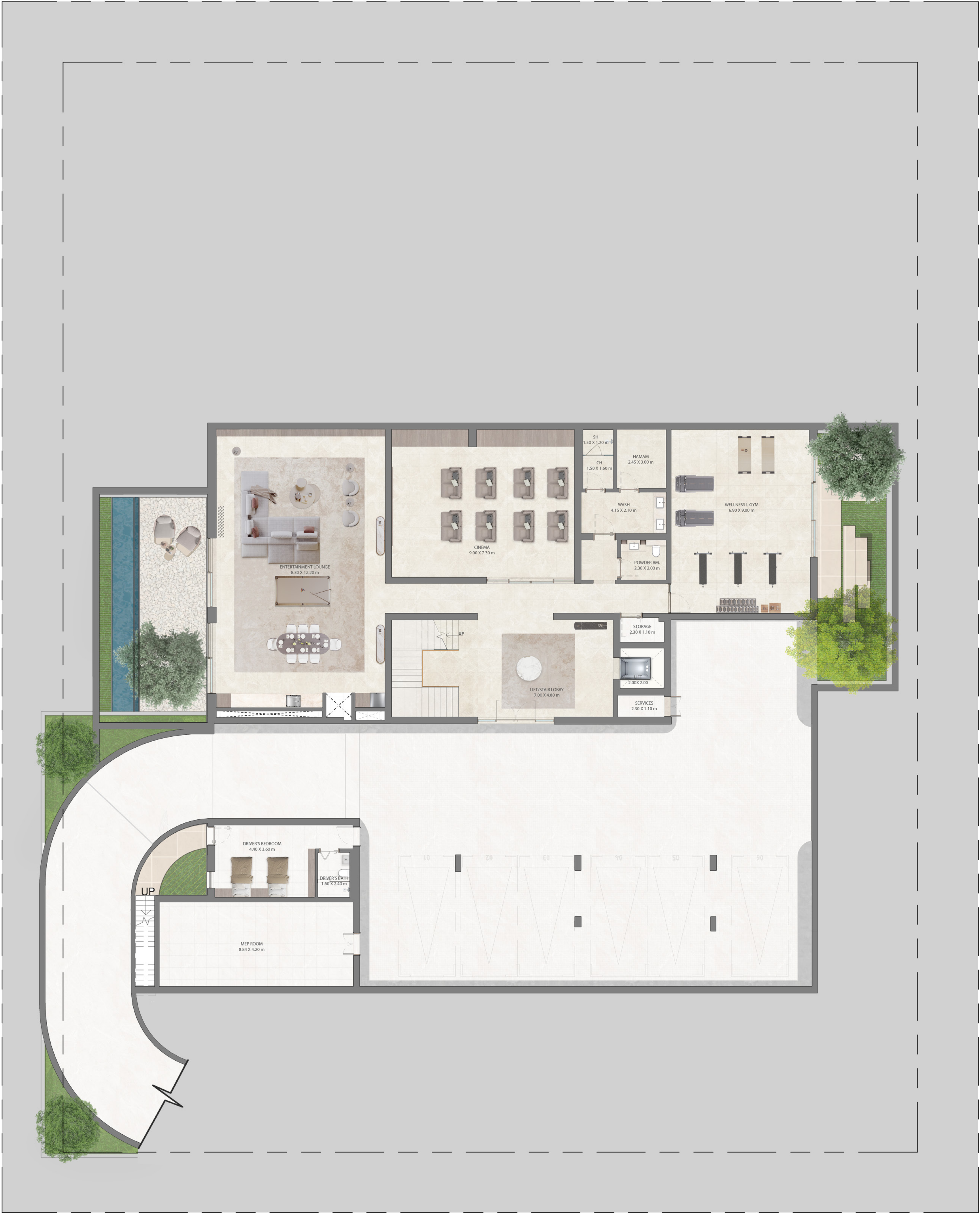
BASEMENT
